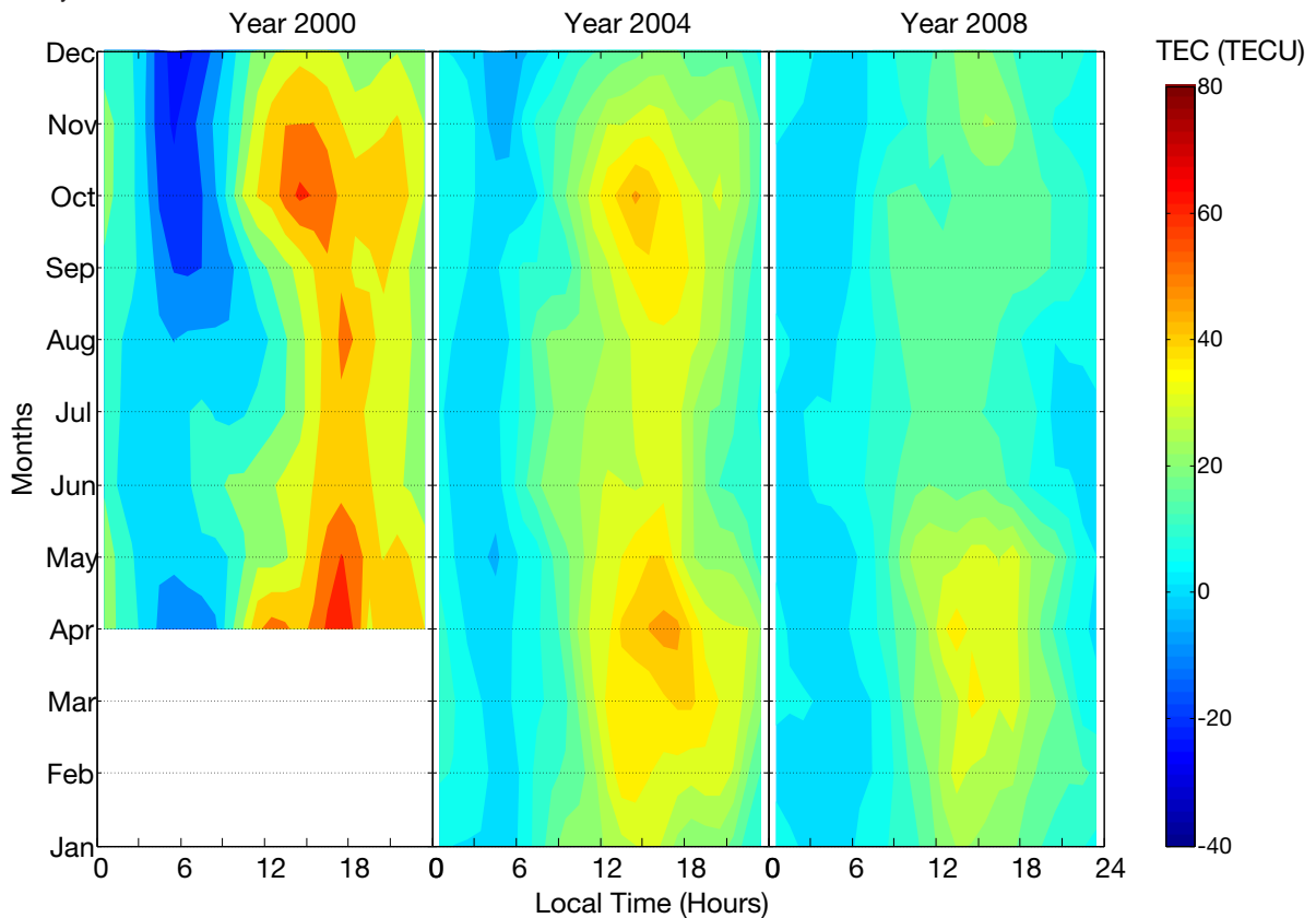
Fig. 10: Monthly mean variations of equivalent EIA at during low, moderate and high solar activity.
