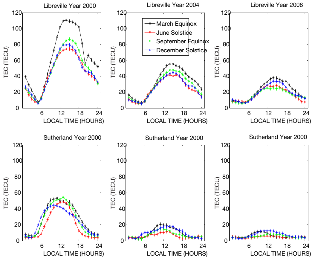
Fig. 9: Seasonal variations of TEC at Libreville and Sutherland during low, moderate and high solar activity.
