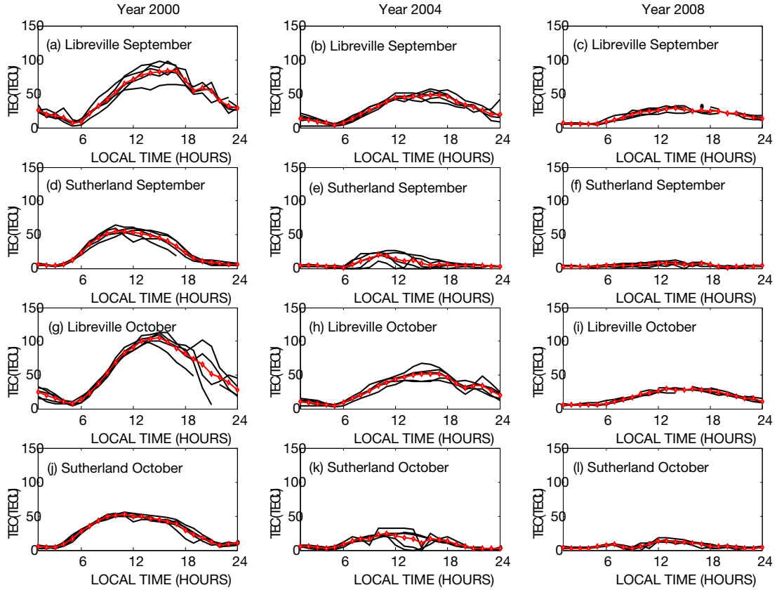
Fig. 5: Five most quiet days and monthly mean of TEC at Libreville and Sutherland in September and October during low, moderate and high solar activity.
