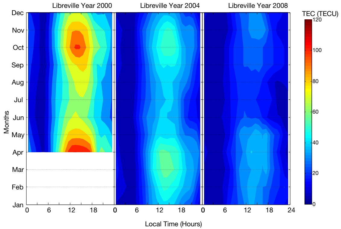
Fig.7: Monthly mean variation of TEC at Libreville.
