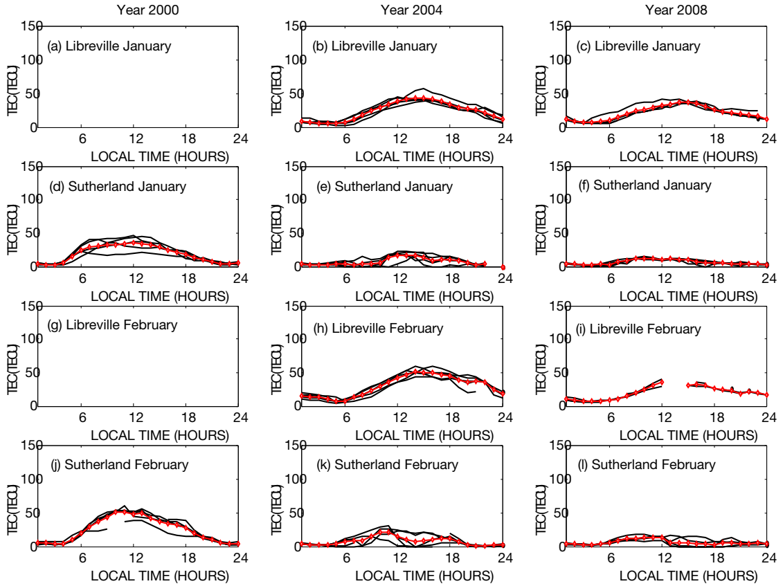
Fig. 1: Five most quiet days and monthly mean of TEC at Libreville and Sutherland in January and February during low, moderate and high solar activity.
