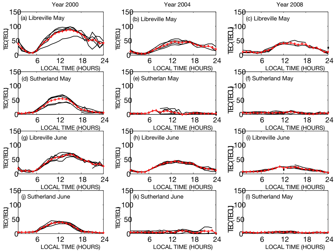
Fig. 3: Five most quiet days and monthly mean of TEC at Libreville and Sutherland in May and June during low, moderate and high solar activity.
