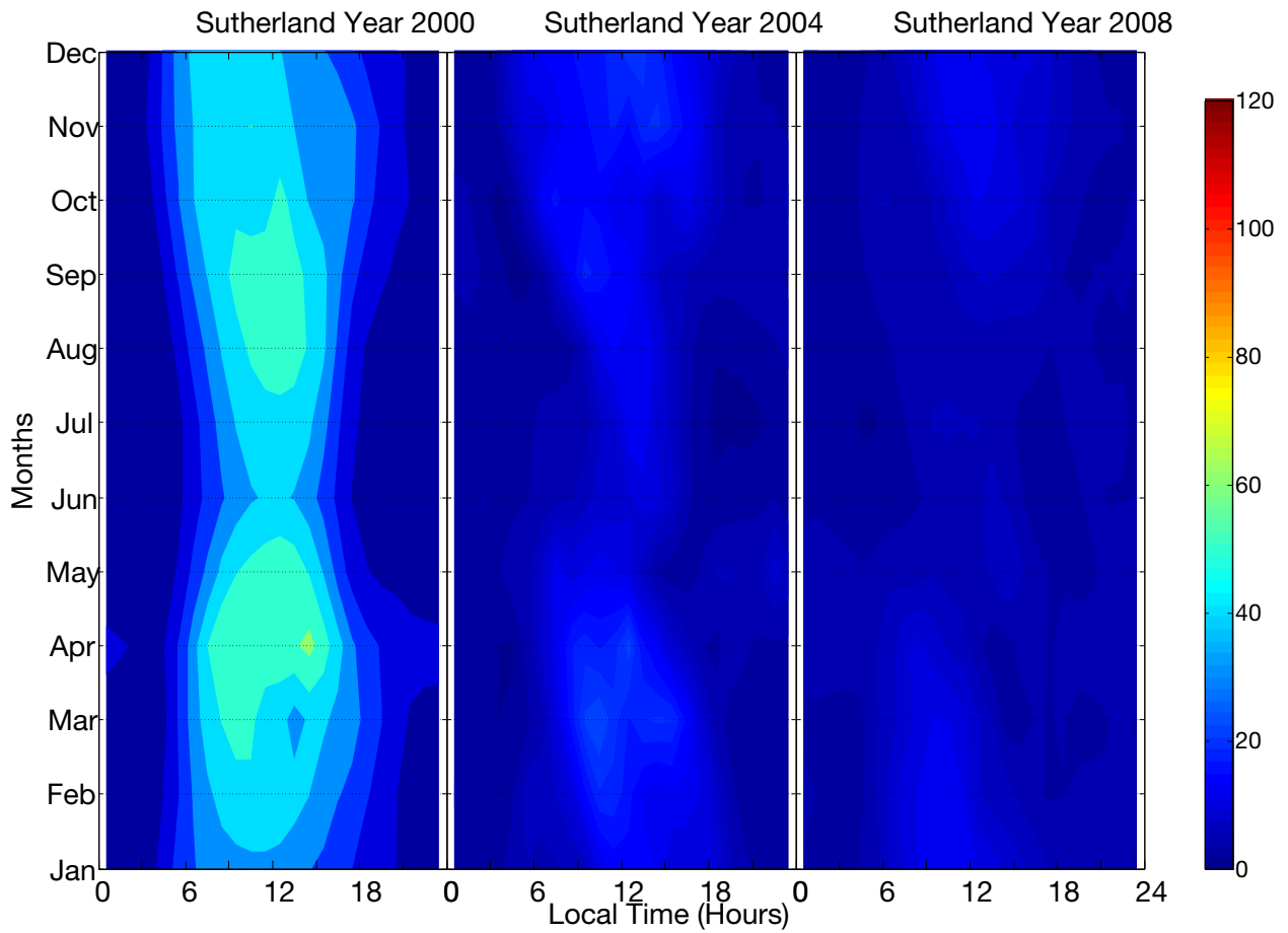
Fig. 8: Monthly mean variation of TEC at Sutherland.
