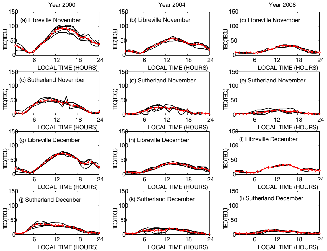
Fig. 6: Five most quiet days and monthly mean variations of TEC at Libreville and Sutherland in November and December during low, moderate and high solar activity.
