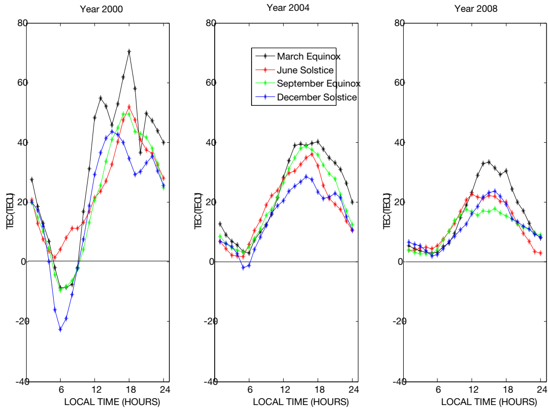
Fig. 11: Seasonal variations of equivalent EIA during low, moderate and high solar activity.
