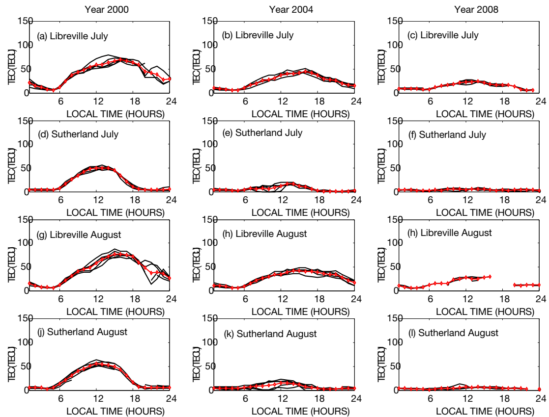
Fig. 4: Five most quiet days and monthly mean of TEC at Libreville and Sutherland in July and August during low, moderate and high solar activity.
