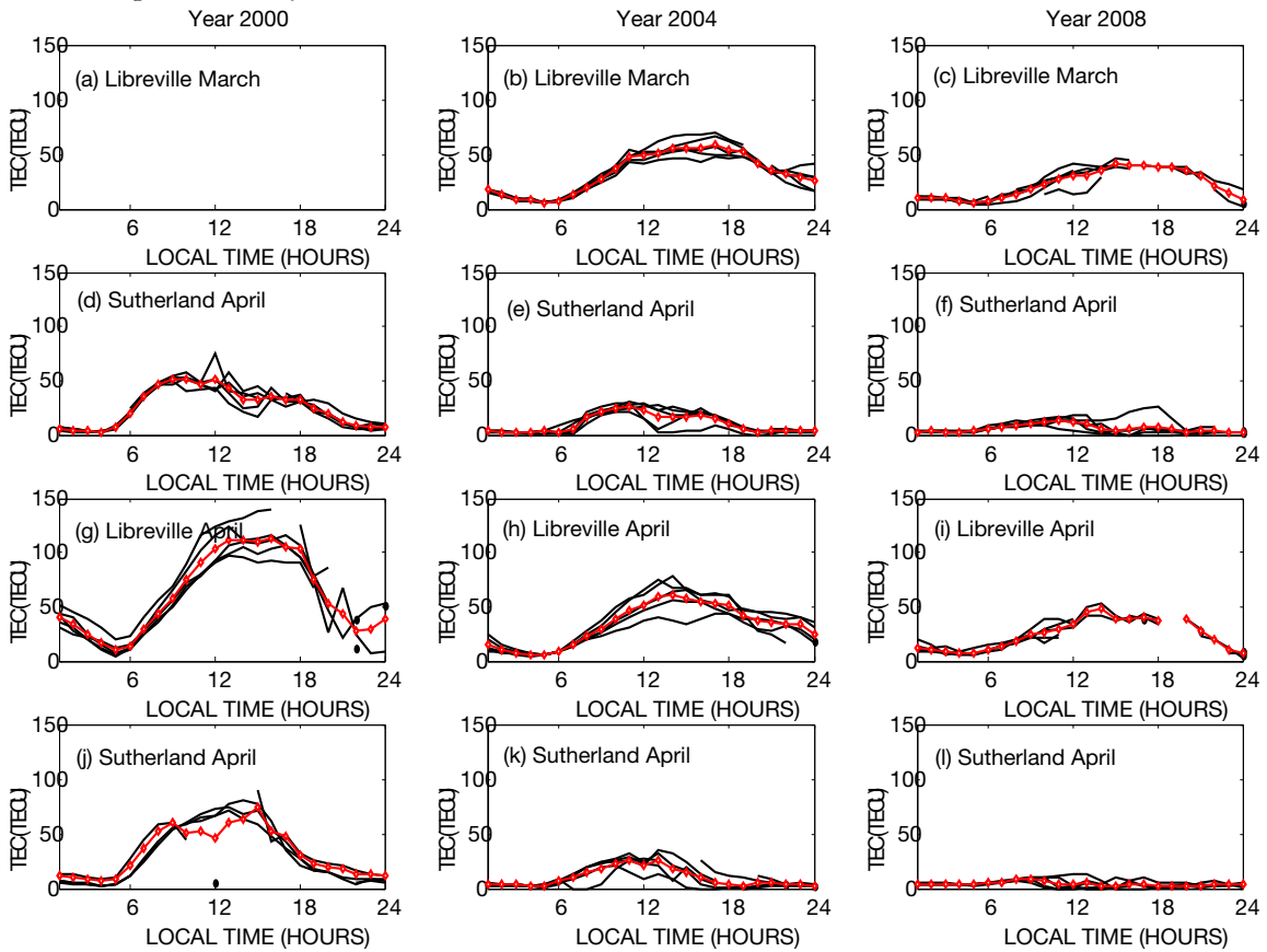
Fig. 2: Five most quiet days and monthly mean of TEC at Libreville and Sutherland in March and April during low, moderate and high solar activity.
